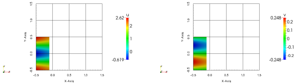
Figure 10.4 Velocity profiles for the Kovaszny Flow in truncated domain (2D).
