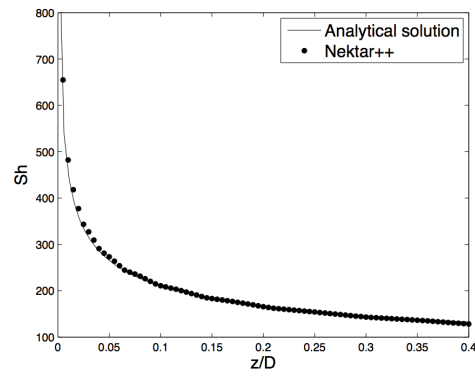
Figure 6.3 Concentration gradient at the surface of the pipe.
