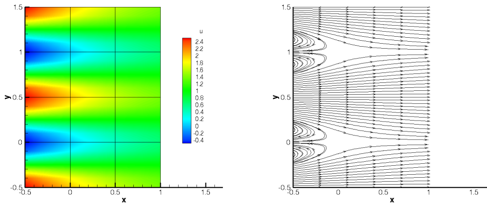
Figure 8.2 Velocity profiles for the Kovaszny Flow (2D).
