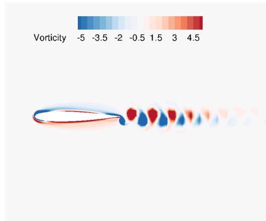
Figure 11.19 Vorticity contour for the self-propelled flapping NACA0012 airfoil.
