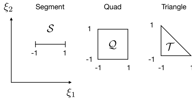
Figure 5.1 Example of the 1D and 2D reference space elements (segment, quad and triangle).
