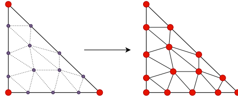
Figure 9.7 Conceptual representation of the creating the LOR space for triangles. The figure on the right shows the LOR space for a higher order triangular element at P=4 , which is viewed as a collocated Lagrange basis at P=1 on \xi_{\text{ele}} points indicated by red dots. The higher-order element on the left currently shows the nodal expansion basis, which is purely for visualisation.
