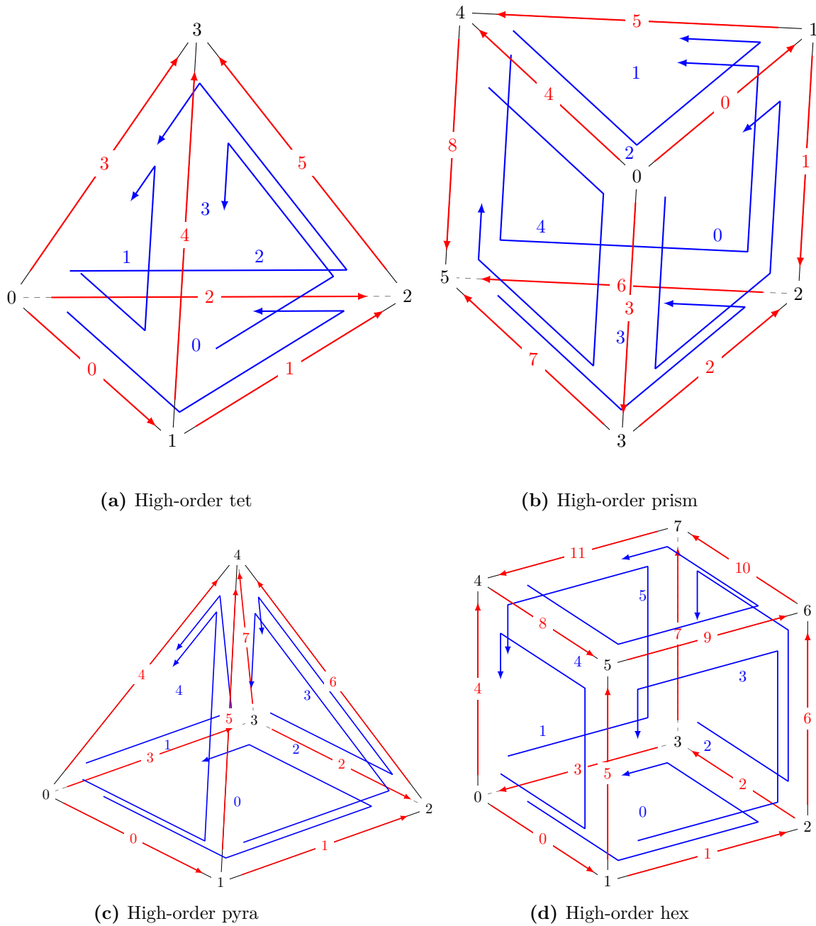
Figure 17.11 Node ordering rules for higher order 3D elements elements
