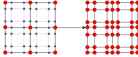
Figure 9.4 Representation of converting a higher-order finite element grid at P=3 to its lower-order P=1 equivalent for the LOR preconditioner. The red dots represent the points on the linear mesh, and the purple dots represent the quadrature points within a linear element. The resulting LOR mesh only contains linear DOF. The spacing of the linear DOF for the LOR mesh here is done in a GLL manner, the same as that of the higher-order element.
