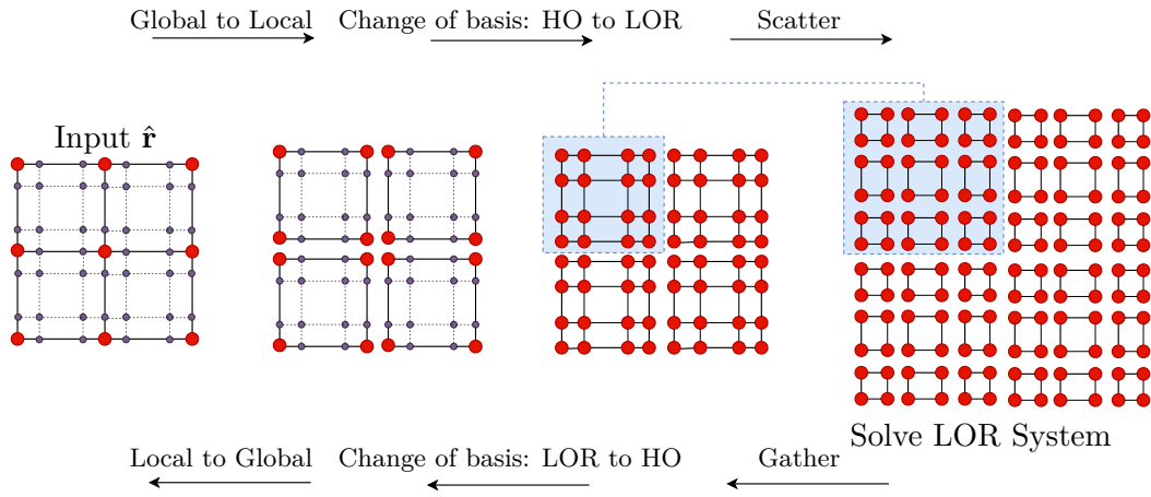
Figure 9.5 Representation of the current algorithm for the LOR preconditioner. There are three major steps: a. The conversion to the LOR mesh (left to right), b. solving the LOR linear system and c. projecting the solution back to the HO mesh (right to left). This process takes place at every preconditioned iteration.
