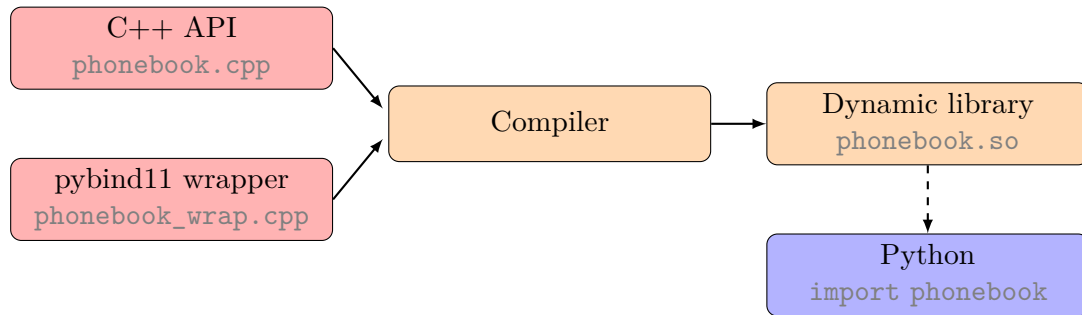
Figure 18.1 A schematic diagram of how C++ code is converted into Python with Boost.Python [51]
