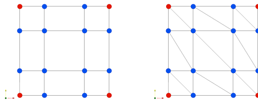
Figure 9.6 Available options for the LOR grids for the quadrilateral elements in 2D. The red dots correspond to the original HO element, and the blue dots are the GLL points in the LOR for P=3 . Left: \mathcal{Q}1 configuration, Right: \mathcal{P}1 configuration.
