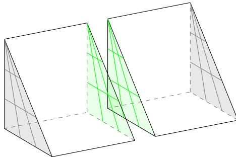
(a) Valid element: neighbouring tri faces are aligned
