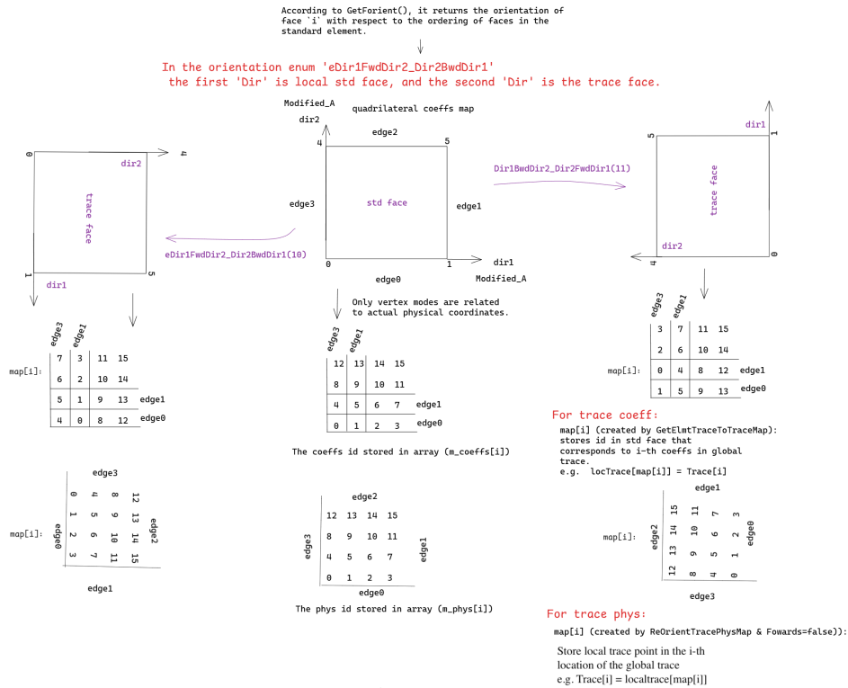
Figure 7.3 Example of trace mappings for complex transposed cases eDir1FwdDir2_Dir2BwdDir1 and eDir1BwdDir2_Dir2FwdDir1 .
