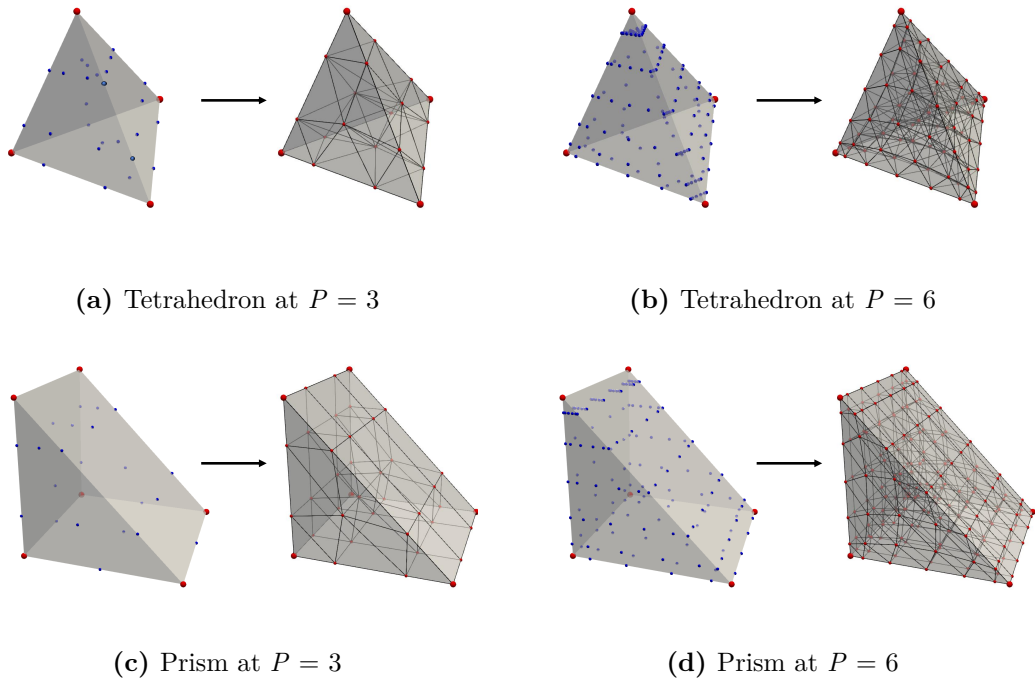
Figure 9.8 Visual representation of the creating the LOR space for simplices at P = 3 and 6. Within each subfigure, the figure on the right shows the LOR space for a HO element on the left. The LOR space is viewed as a collocated Lagrange basis at P=1 indicated by red dots, with on \xi_{\text{ele}} points in the interior and \xi_{\text{GLL}} points constrained the boundary. One can identify this by looking at any of the triangular faces for the simplices.
