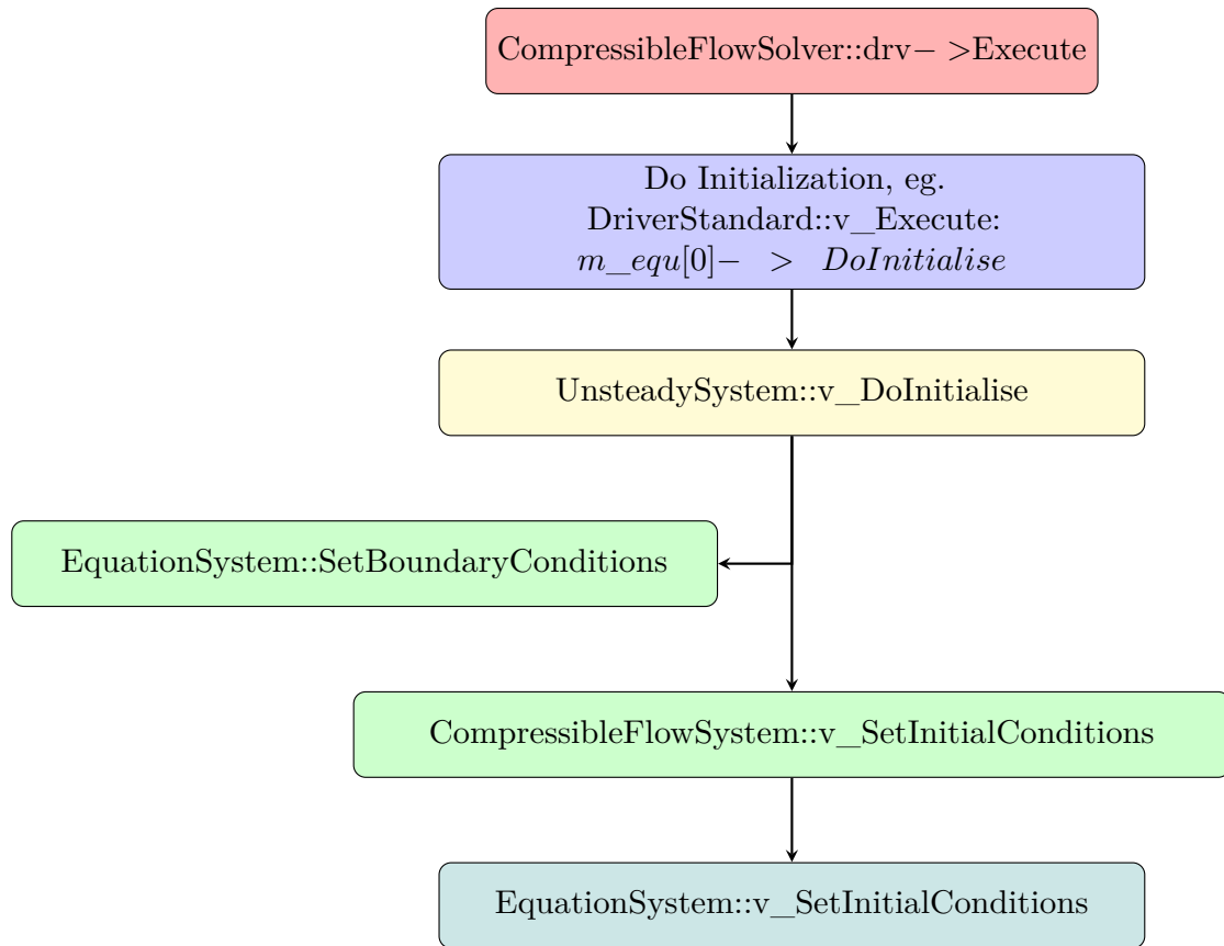
Figure 15.4 CompressibleFlowSolver Initialize Conditions
