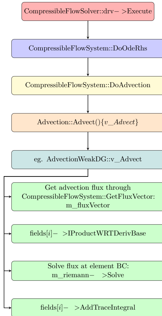
Figure 15.5 CompressibleFlowSolver Execute Advection
