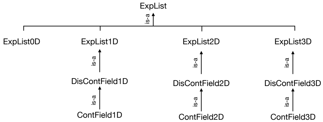
Figure 9.3 Class hierarchy derived from ExpList , the base class of the MultiRegions Directory.
