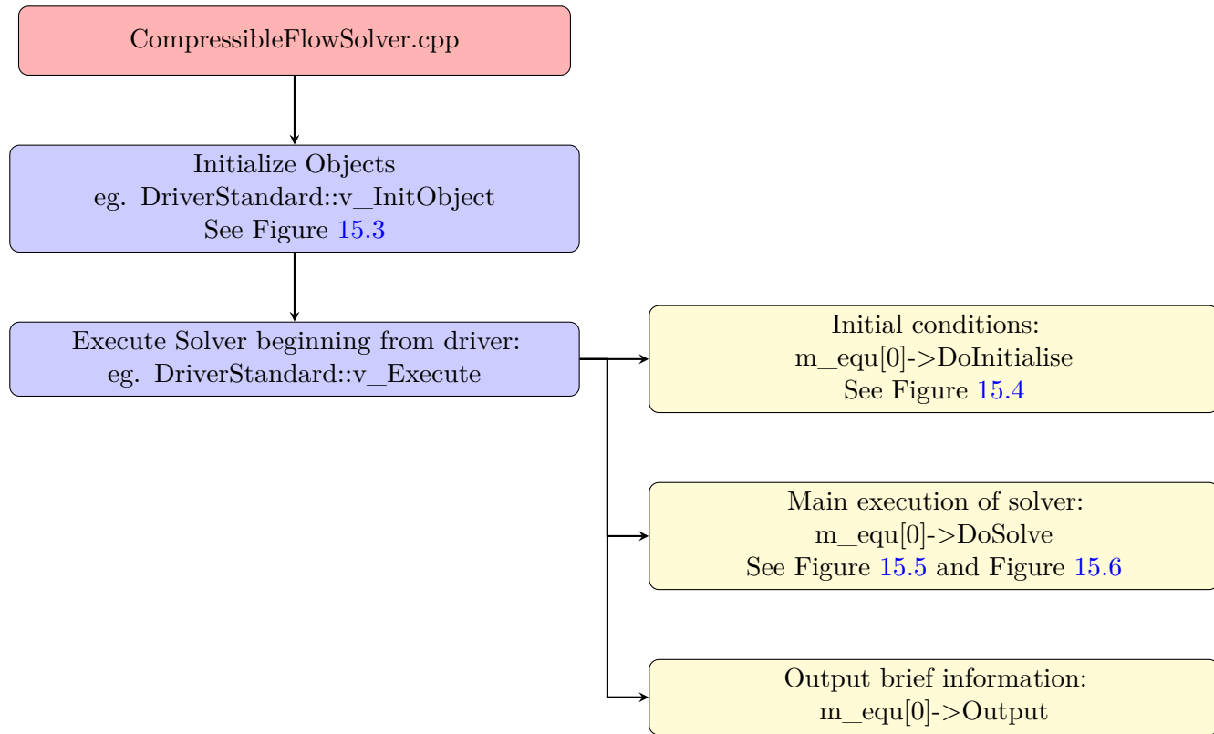
Figure 15.2 CompressibleFlowSolver Main Flow Chart
