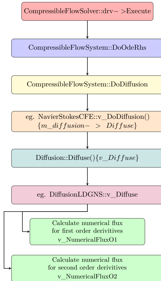
Figure 15.6 CompressibleFlowSolver Execute Diffusion
