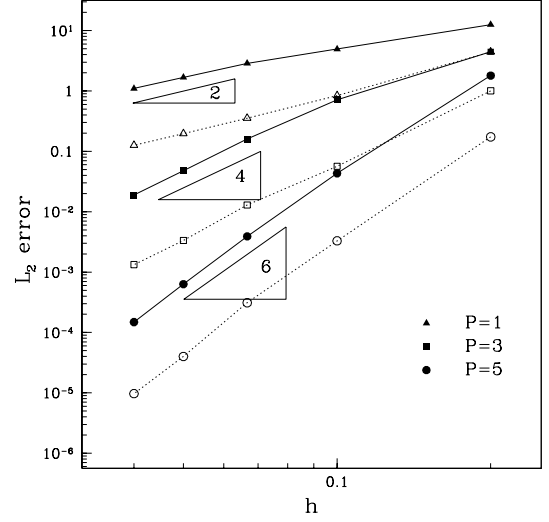
Fig. 9. L_2 error of the solution to the Poisson problem as a function of mesh size h for different polynomial expansions on (a) quadrilateral and (b) triangular mesh. The solid lines denote the HDG solution with \tau = 1 and the dotted lines represent the HDG solution with \tau = 1000 .
