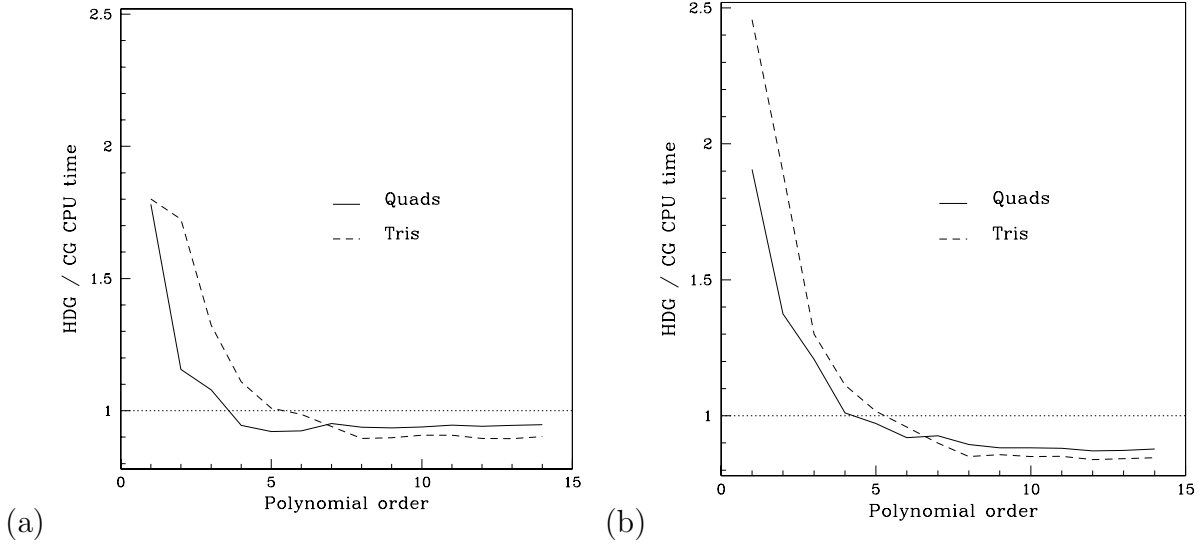
Fig. 7. Relative CPU time of the HDG versus CG solve times as a function of polynomial order for the quadrilateral mesh (solid line) and the triangular mesh (dashed line). (a) 15 \times 15 mesh, (b) 25 \times 25 mesh. The dotted line indicates equivalent speed.
