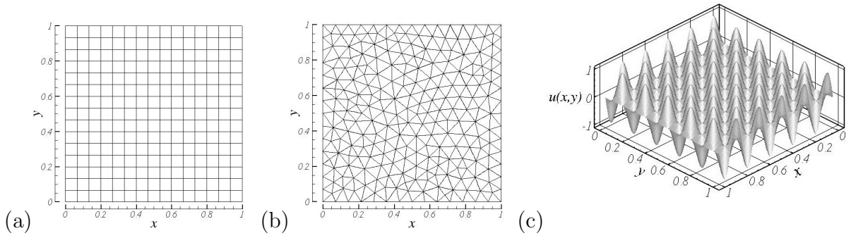
Fig. 5. Discretizations of the unit square where each edge is divided into 15 segments using (a) regular quadrilateral regions and (b) unstructured triangular regions. A representative solution field u(x,y) = \sin(10\pi x)\cos(10\pi y) is shown in Figure (c)
