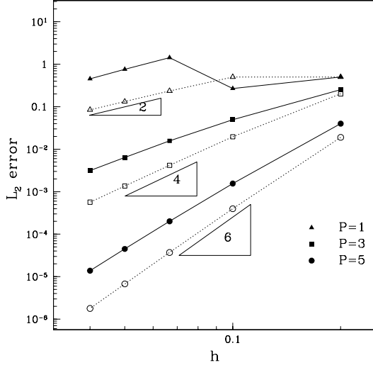
Fig. 9. L_2 error of the solution to the Poisson problem as a function of mesh size h for different polynomial expansions on (a) quadrilateral and (b) triangular mesh. The solid lines denote the HDG solution with \tau = 1 and the dotted lines represent the HDG solution with \tau = 1000 .
