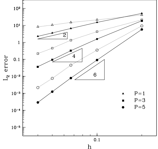
Fig. 10. L_2 error of the weak discontinuous Galerkin flux q to the solution to the Poisson problem as a function of mesh size h for different polynomial expansions on (a) quadrilateral and (b) triangular mesh. The solid lines denote the HDG solution with \tau = 1 and the dotted lines represent the HDG solution with \tau = 1000 .
