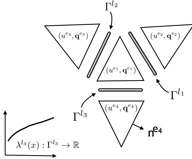
Fig. 3. Diagram showing the relationship between the local solutions and the trace-space variables.
