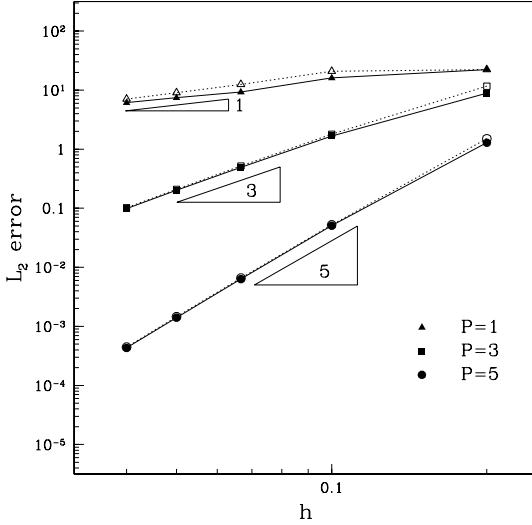
Fig. 10. L_2 error of the weak discontinuous Galerkin flux q to the solution to the Poisson problem as a function of mesh size h for different polynomial expansions on (a) quadrilateral and (b) triangular mesh. The solid lines denote the HDG solution with \tau = 1 and the dotted lines represent the HDG solution with \tau = 1000 .
