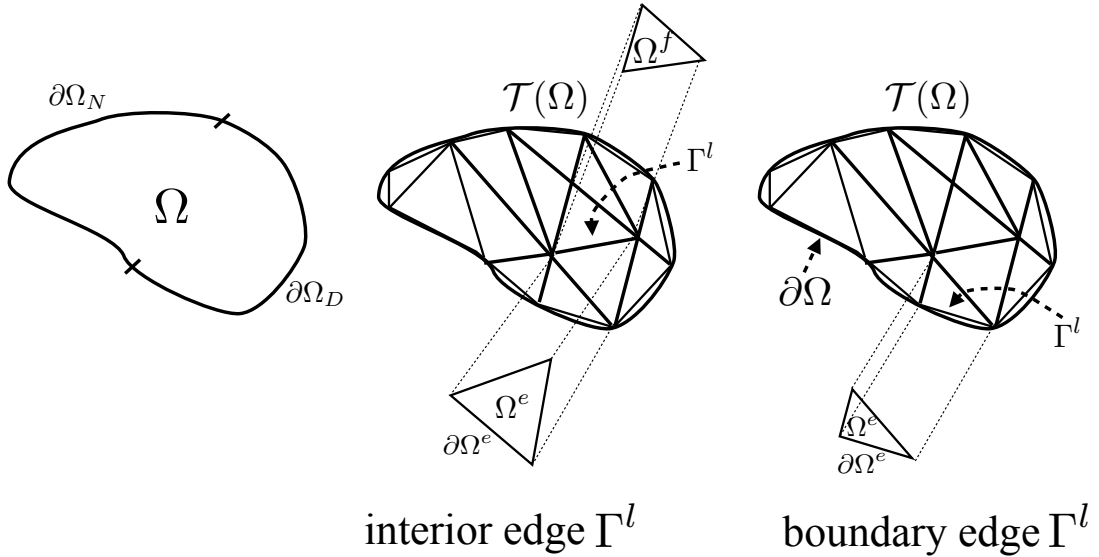
Fig. 1. Diagram of the domain and corresponding tessellation demonstrating the use of our notation.
