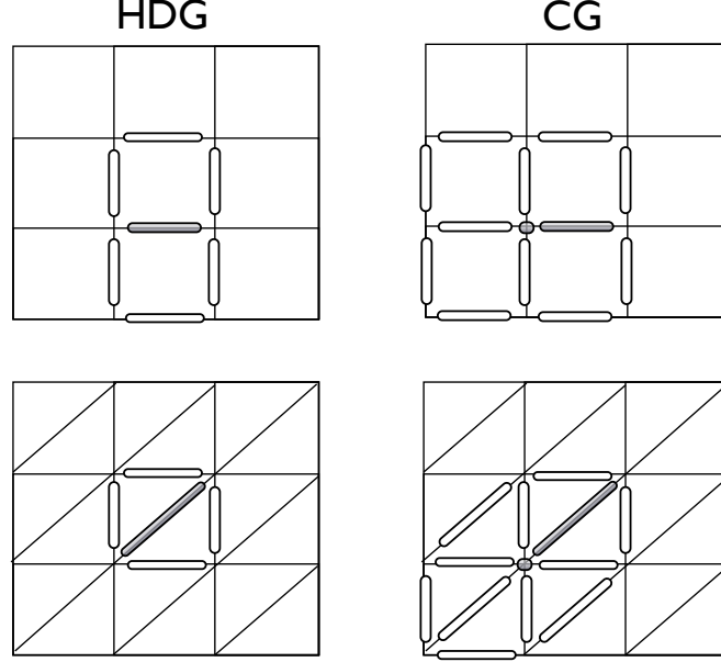
Fig. 8. Schematic of coupling of an edge in HDG and edge plus a vertex for CG with adjacent edges. The coupled degrees of freedom are identified by a shaded long oval and the edges that are connected to this edge are identified by white ovals.
