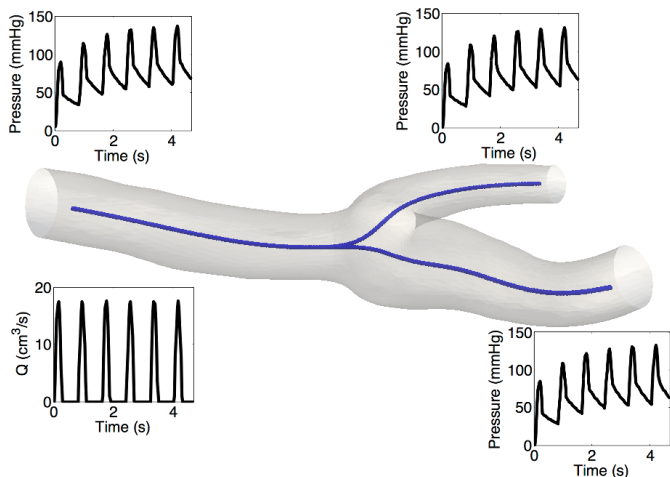
Figure 9: Geometry used for the simulation. Insets show how flow and pressure vary with time and different locations in the geometry. Simulation input files are provided in Appendix A.22.
