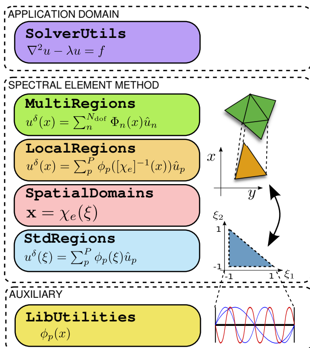
Figure 1: Nektar++ architecture diagram. Shows the relationship between the individual libraries in the framework and the mathematical constructs to which they relate.
