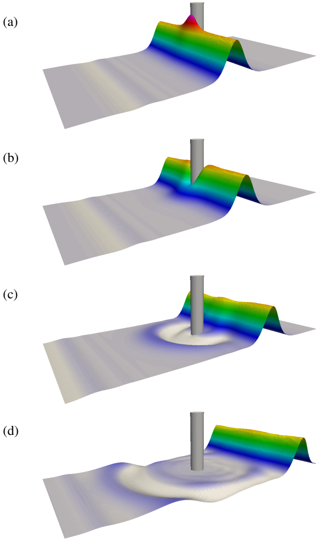
Figure 7: Solitary wave impinging a stationary cylinder. The colours and surface deformation illustrate the height of the surface at times (a) t = 4.5\text{s} ; (b) t = 5.5\text{s} ; (c) t = 8.5\text{s} ; and (d) t = 12.5\text{s} . Simulation input files are provided in Appendix A.20.
