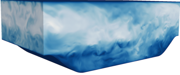
Figure 5: Contours of velocity magnitude in a periodic hill simulation at Re = 2800 . Simulation input files available in Appendix A.18
