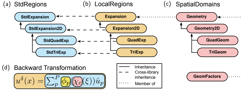
Figure 2: Example of class inheritance structure for two-dimensional regions. Each LocalRegions class (b) inherits base functionality from the corresponding StdRegions class (a). Inheritance is used to minimise code duplication. The Expansion class contains member pointers to Geometry and GeomFactors objects (c). Operations, such as a transform from coefficient to physical space (d), on a physical element are constructed as a composition of functionality from the different libraries.
