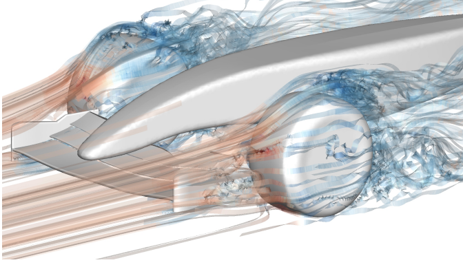
Figure 3: Flow past a front section of a Formula 1 racing car at a Reynolds number of 2.2 \times 10^5 . Streamlines show the flow trajectory and are coloured by pressure. The simulation has 13 million degrees of freedom at polynomial order P = 3 .
