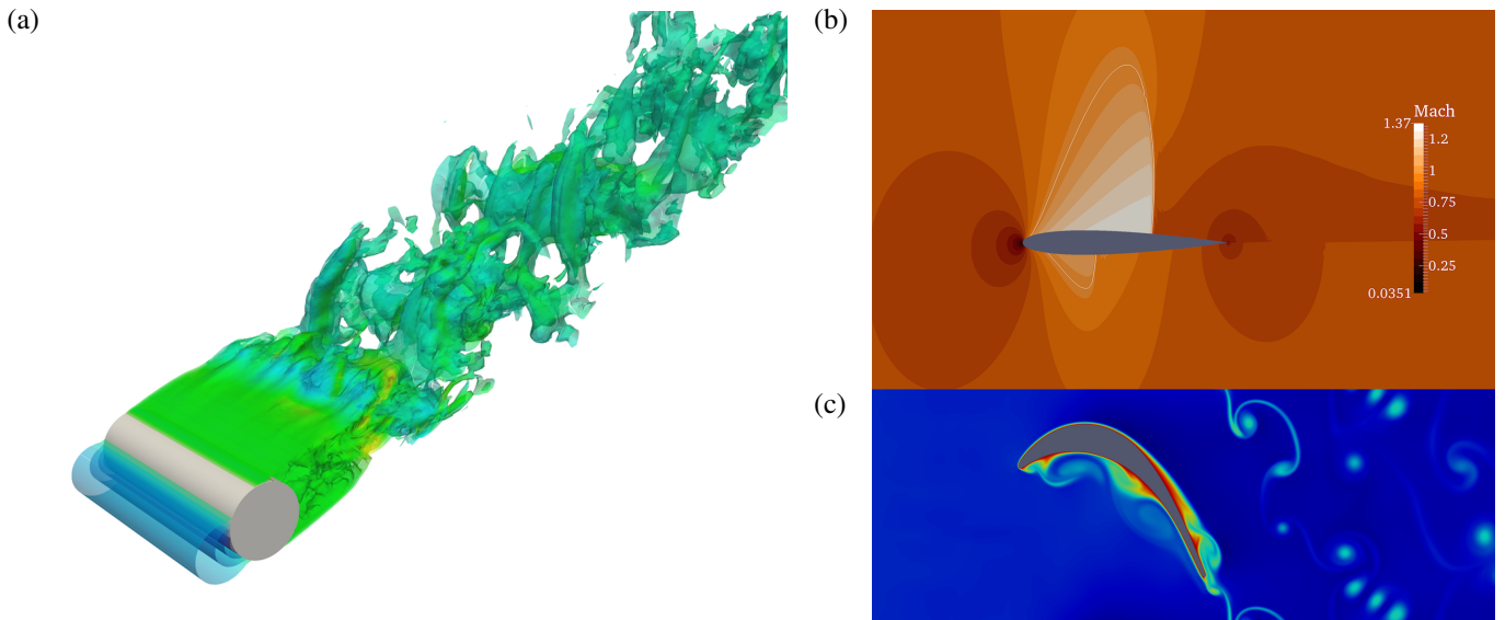
Figure 4: Examples of external aerodynamics problems solved using the CompressibleFlowSolver . (a) Flow over a cylinder at Re = 3,900 . (b) Euler simulation of flow over a NACA0012 aerofoil at Ma_\infty = 0.8 . (c) Temperature of flow passing over a T106C low-pressure turbine blade at Re = 80,000 . Simulation input files are provided in Appendices A.15, A.16 and A.17, respectively.
