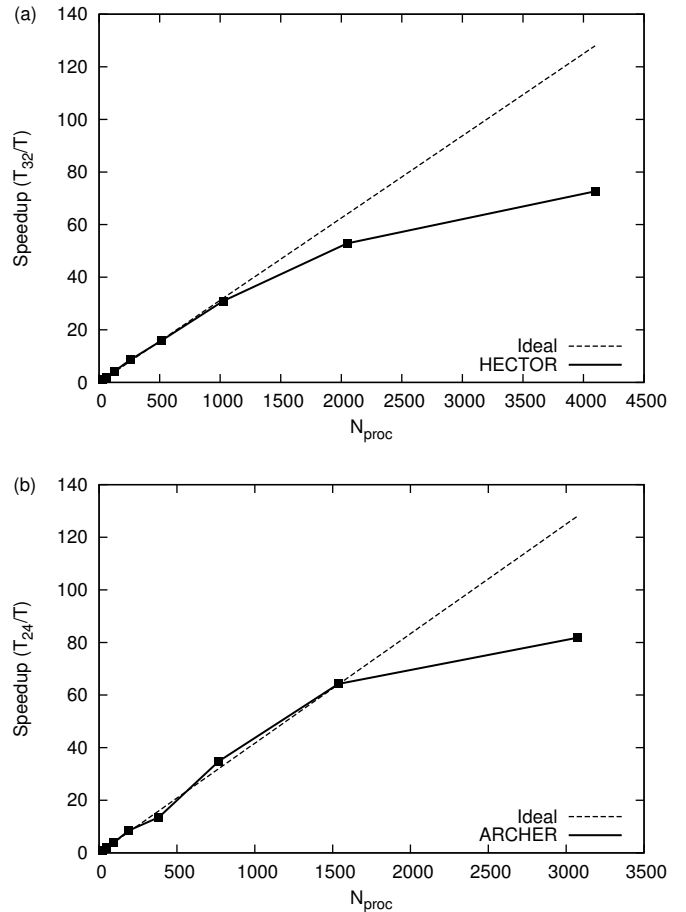
Figure 11: Strong scaling of the Nektar++ diffusion solver on an intercostal pair simulation similar to the one presented in section 4.7. (a) Performance scaling on HECTOR where each node has 32 cores and (b) performance scaling on ARCHER where each node has 24 cores. In both cases, results are normalised by the performance on a single node.
