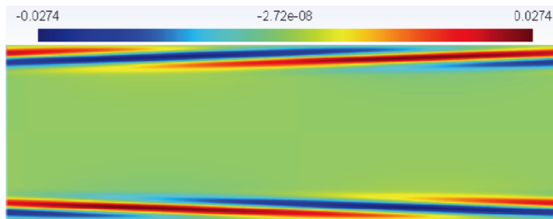
Figure 11.12 u-field of the leading adjoint mode in channel flow at Re = 7500
