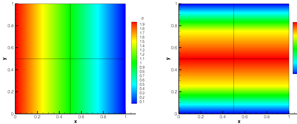
Figure 11.8 Pressure and velocity profiles for the laminar channel flow (2D).
